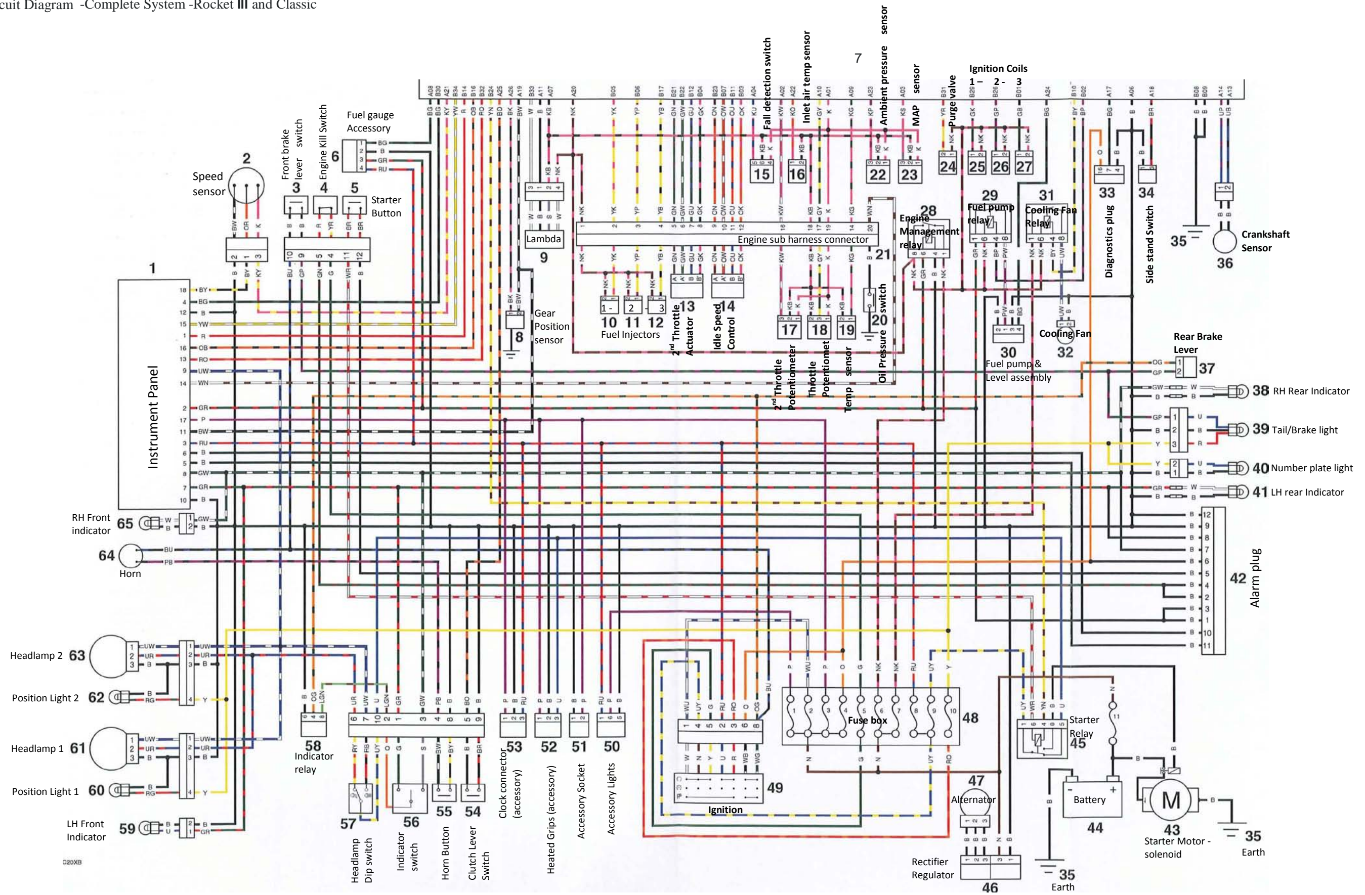
Circuit Diagram -Complete System -Rocket III and Classic
